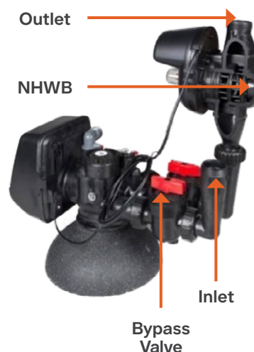
Fig. D V3070FM. Shown with optional V3191-01 vertical adapter kit
